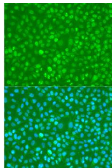
Fig. 4. Immunofluorescence analysis of U2OS cells using Phospho-NF-kB p65-S276 antibody at dilution of 1:100. Blue: DAPI for nuclear staining.
