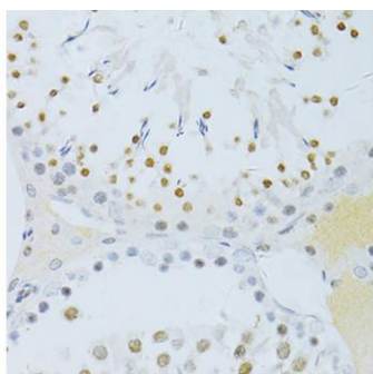
Fig. 3. Immunohistochemistry of paraffin-embedded rat testis using Phospho-NF-kB p65-S276 antibody at dilution of 1:100 (40x lens).
